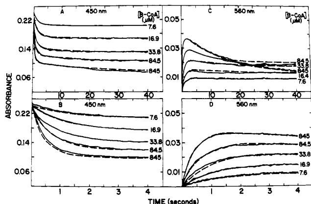
FIGURE 2: Rapid phases in the reduction of oxidized GAD by butyryl-CoA. Conditions: oxidized GAD (16.4 \mu\text{M} ) was anaerobically mixed with butyryl-CoA (15.2–1690 \mu\text{M} ) in 50 mM potassium phosphate buffer, pH 7.6 at 4 ^{\circ}\text{C} , with a stopped-flow spectrophotometer (2-cm optical path length). The panels show the time course of the reaction: (A) at 450 nm, over 40 s; (B) at 450 nm, over 4 s; (C) at 560 nm, over 40 s; (D) at 560 nm, over 4 s. The concentrations of butyryl-CoA (B-CoA) after mixing are indicated opposite each trace. The solid lines are the measured time courses. The dashed lines are simulations based on the scheme in eq 4, using the parameters in Tables I and II.
